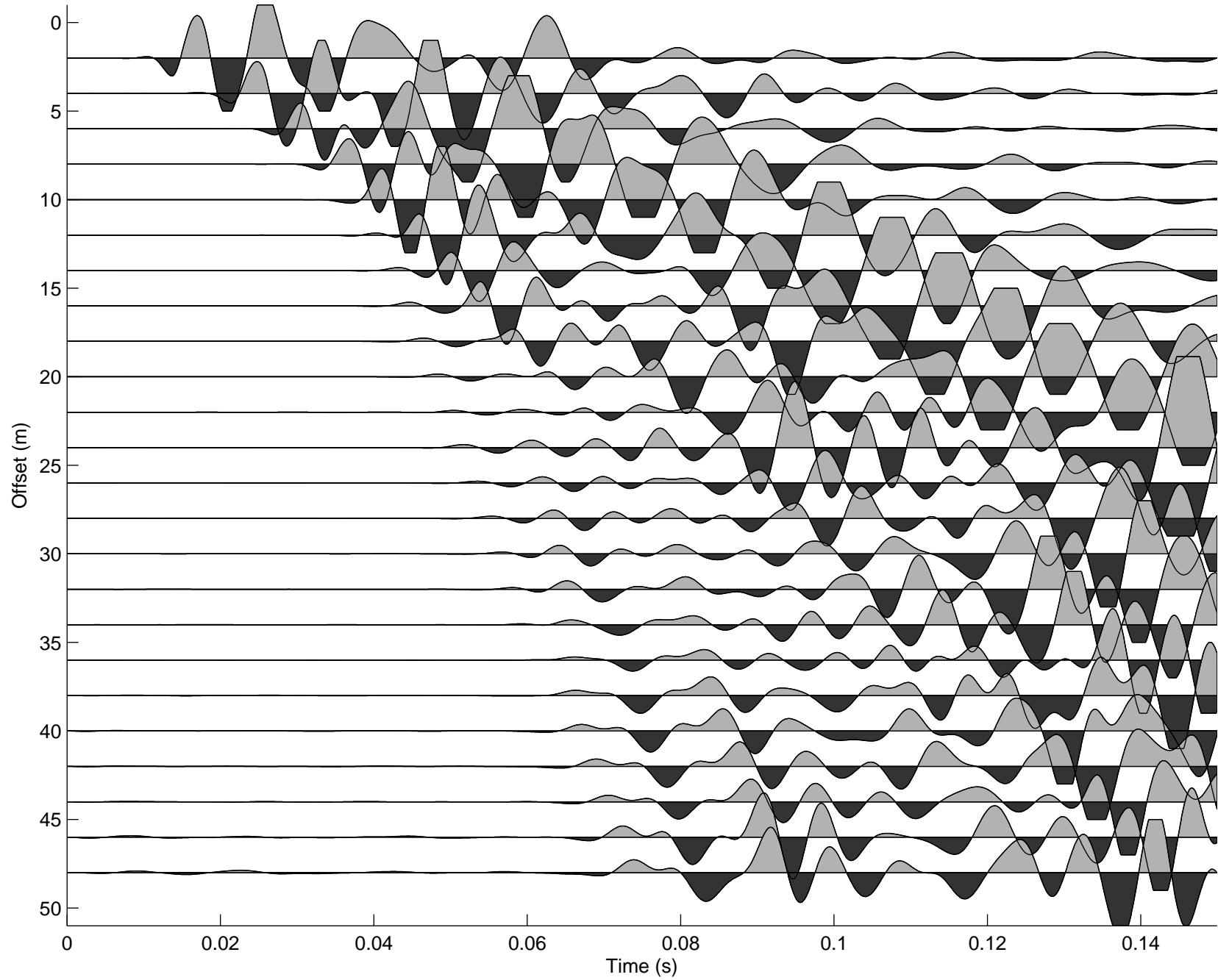
5.dat filtered in band 50–150Hz
