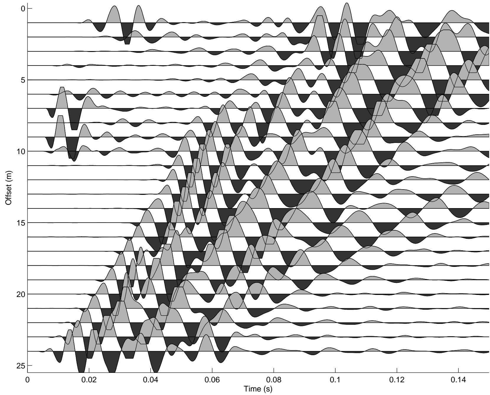
8.dat filtered in band 50–150Hz
