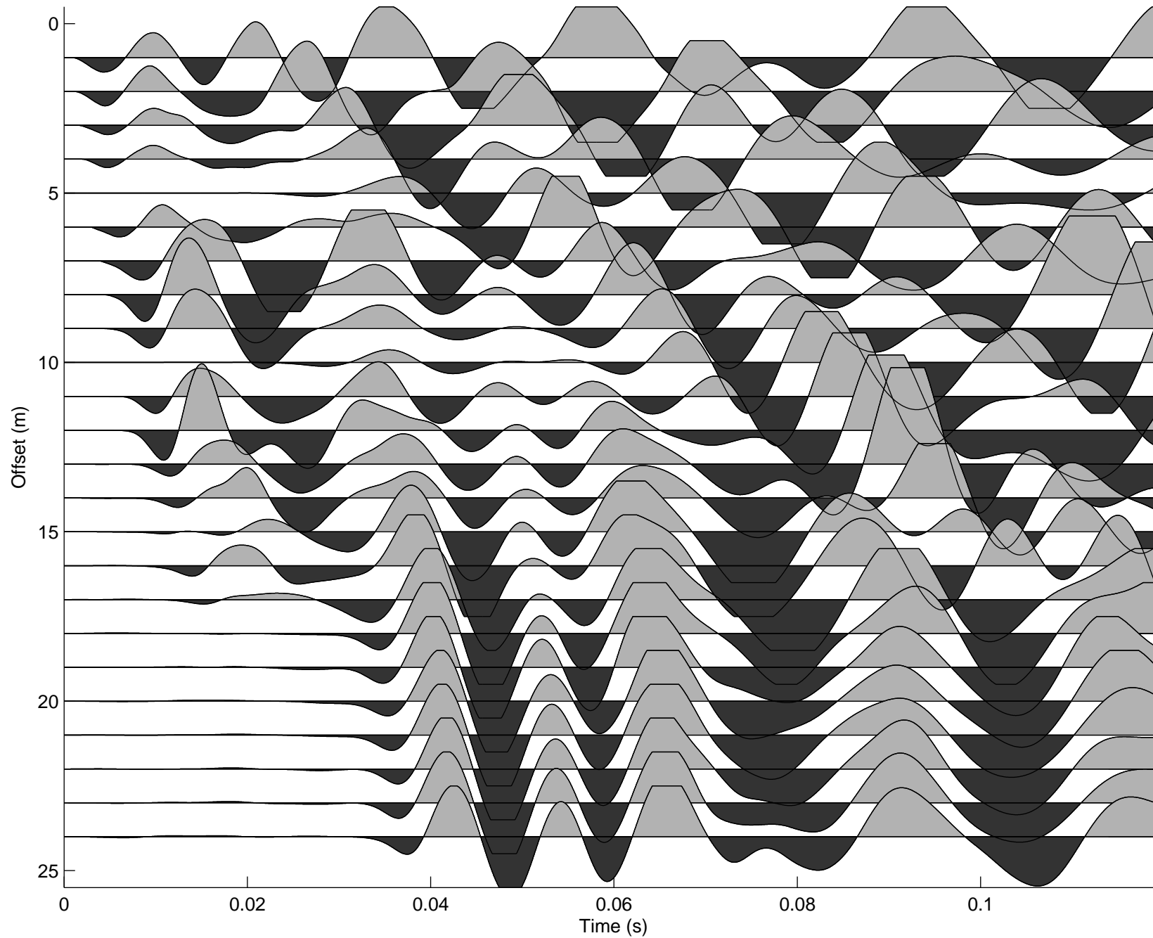
201.dat filtered in band 20–80Hz
