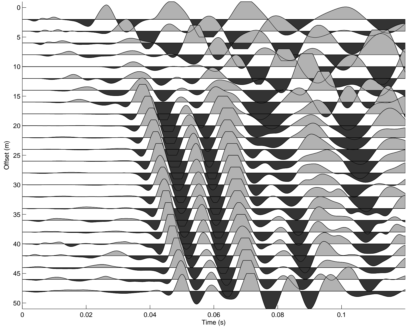
205.dat filtered in band 20–80Hz
