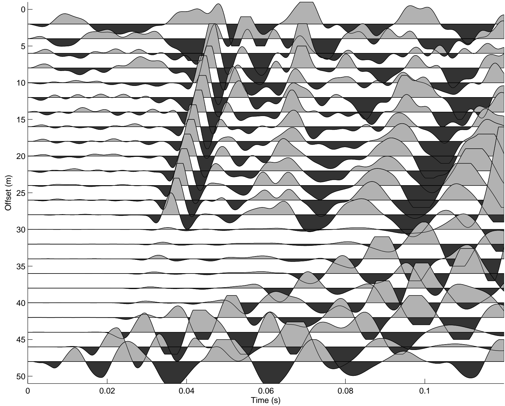
208.dat filtered in band 20–80Hz
