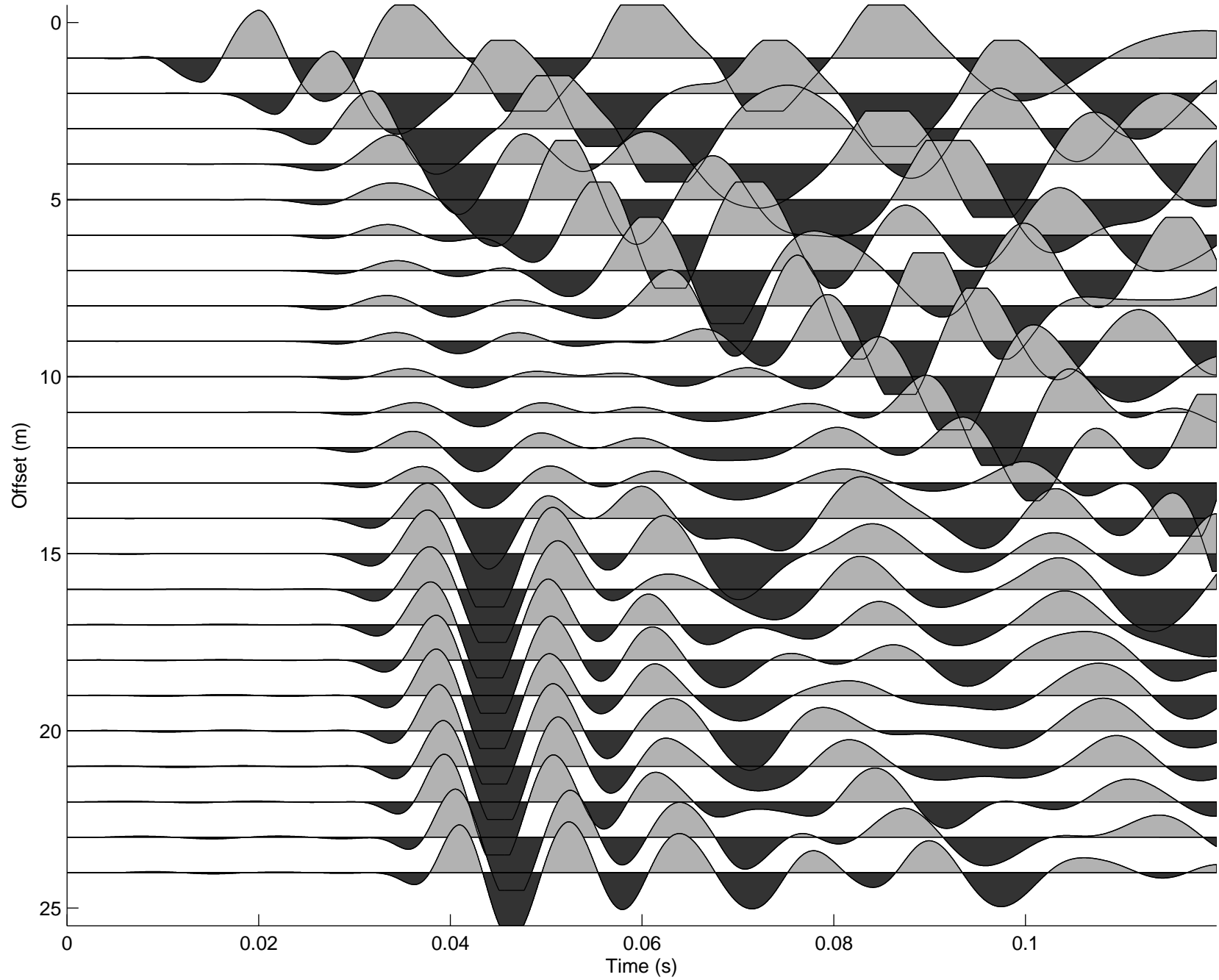
210.dat filtered in band 20–80Hz
