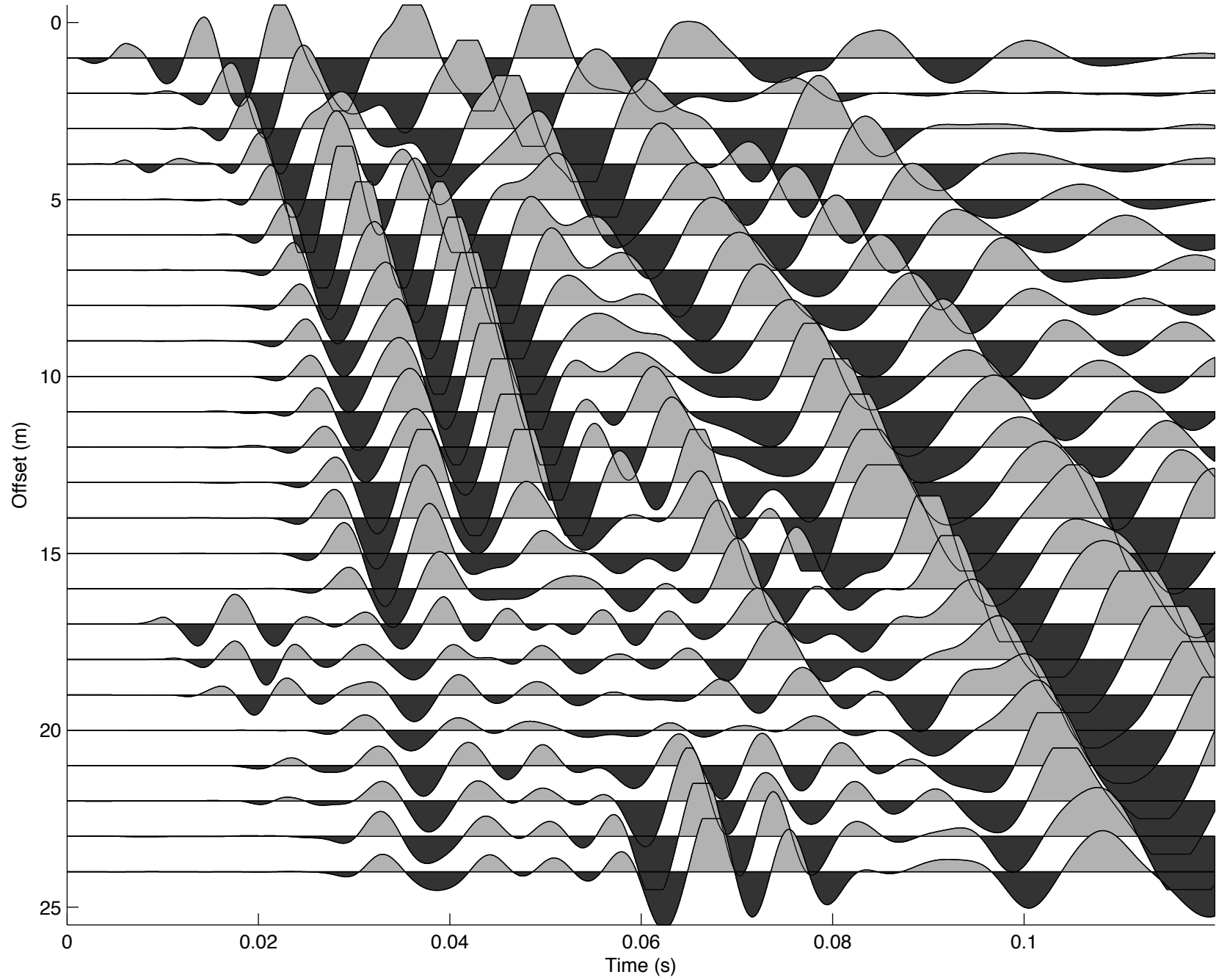
301.dat filtered in band 50–150Hz
