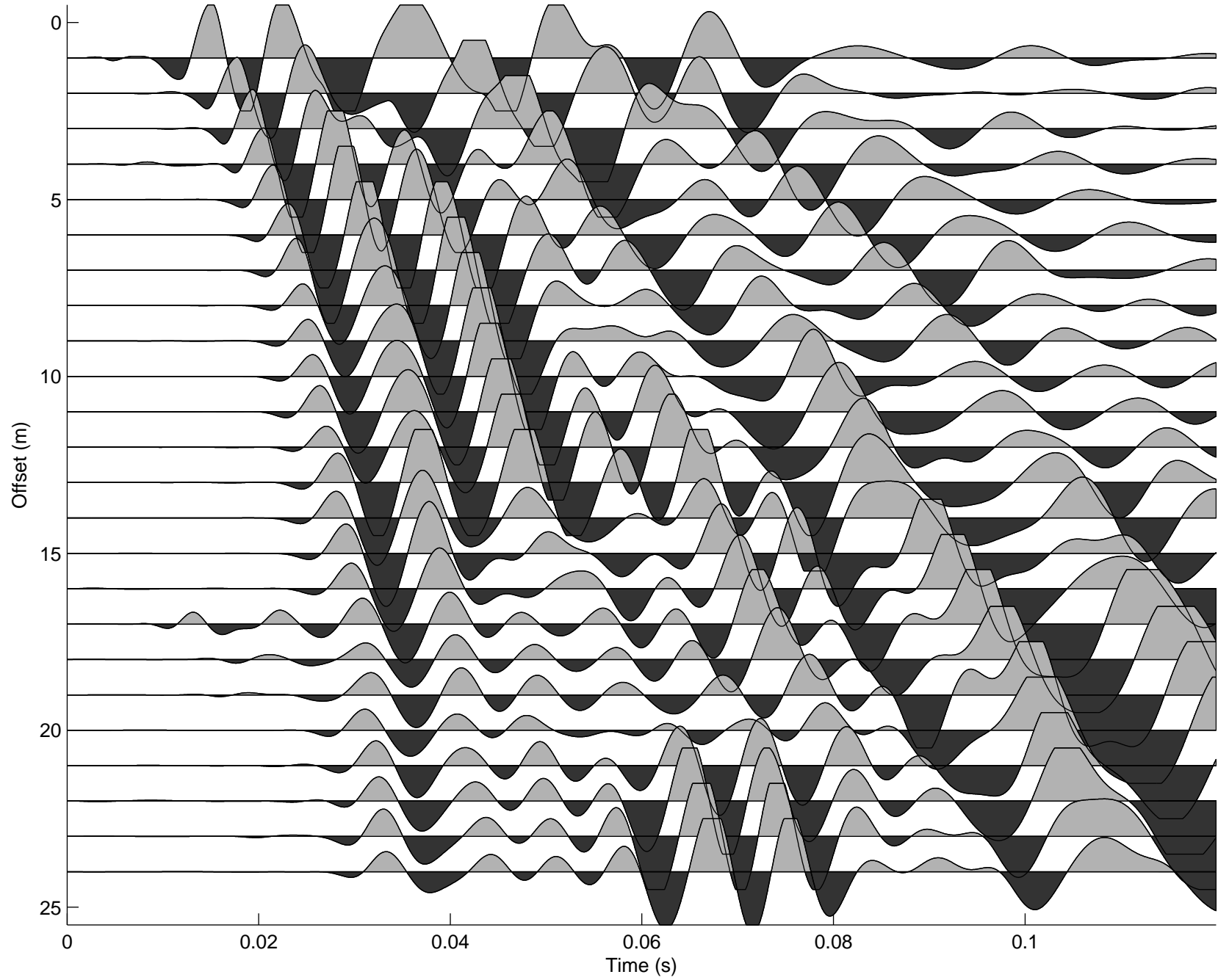
302.dat filtered in band 50–150Hz
