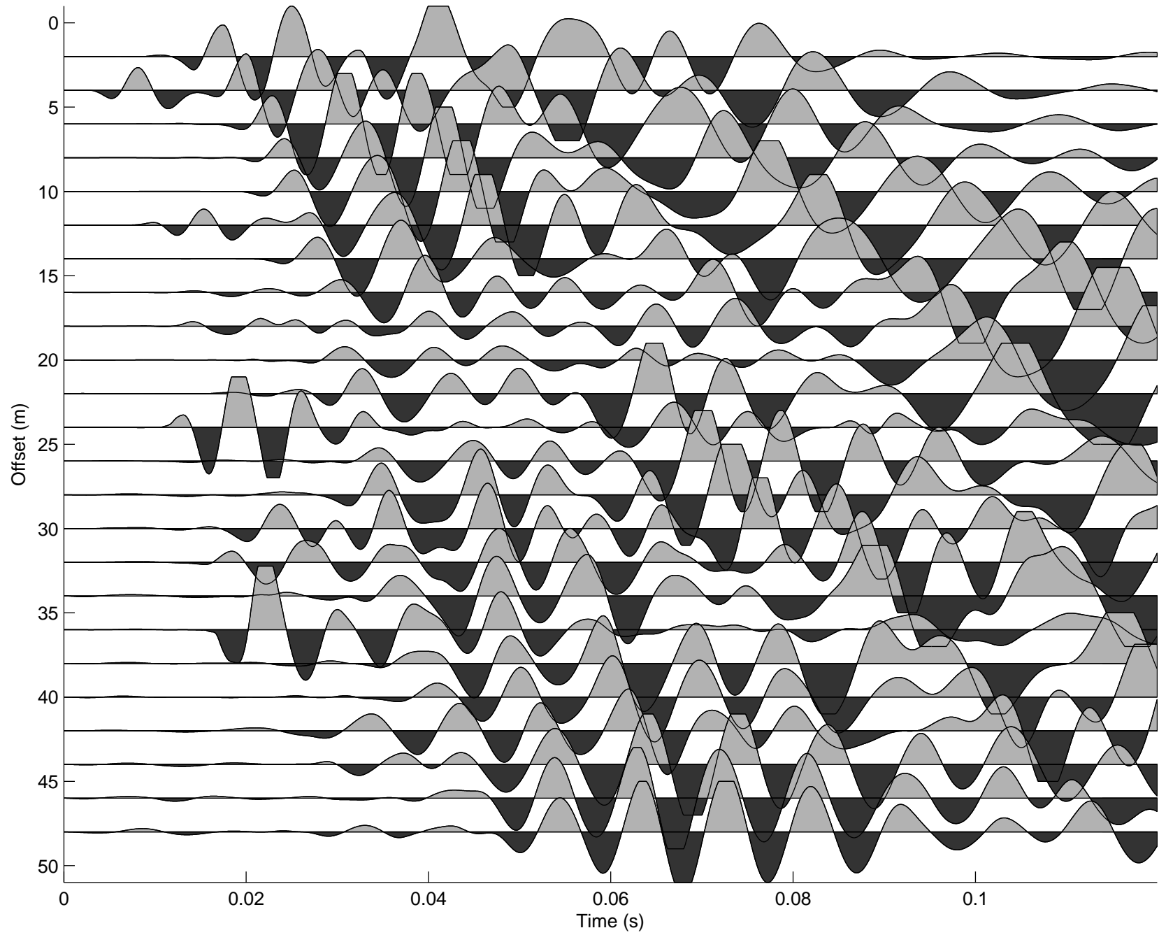
306.dat filtered in band 50–150Hz
