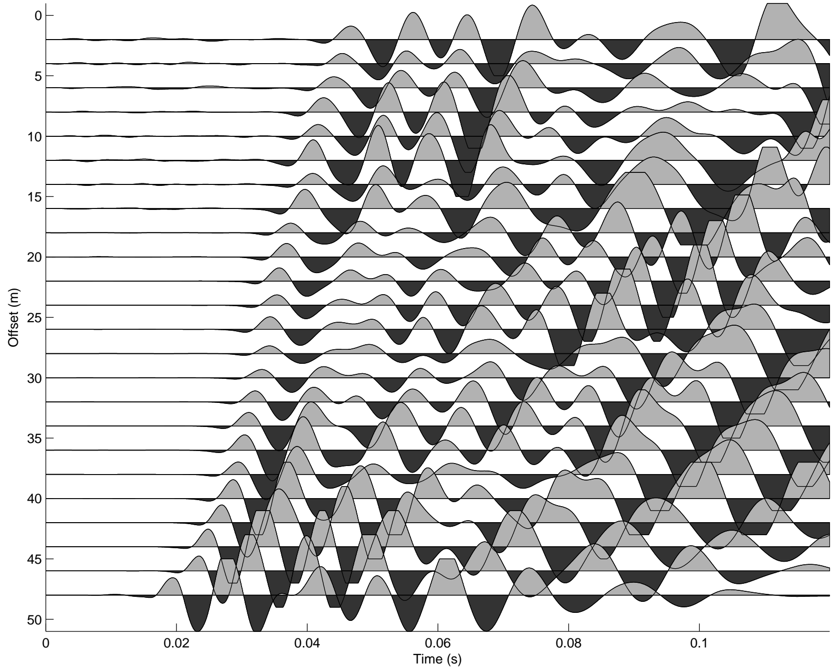
312.dat filtered in band 50–150Hz
