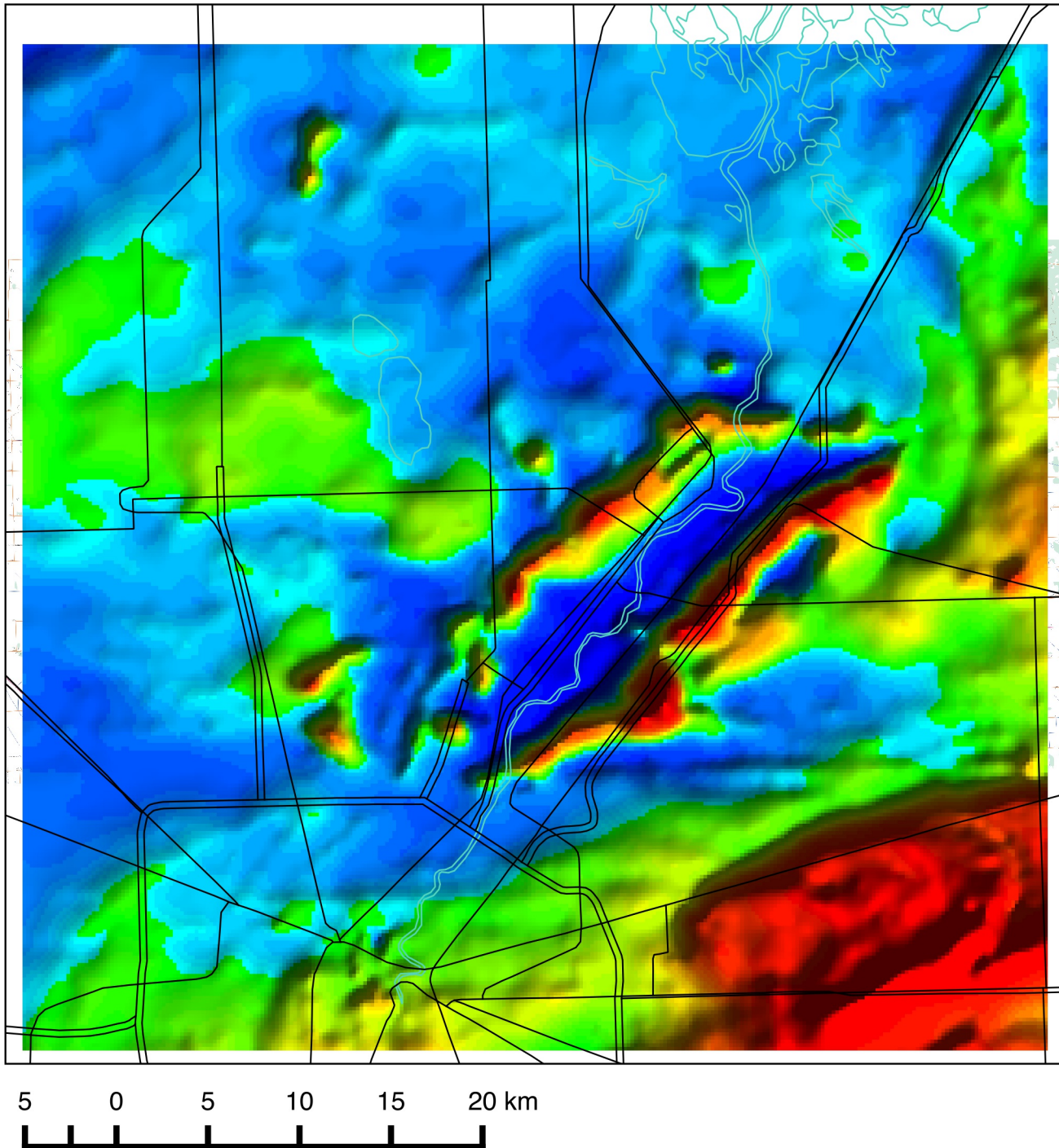
Total field magnetics (shaded relief)
