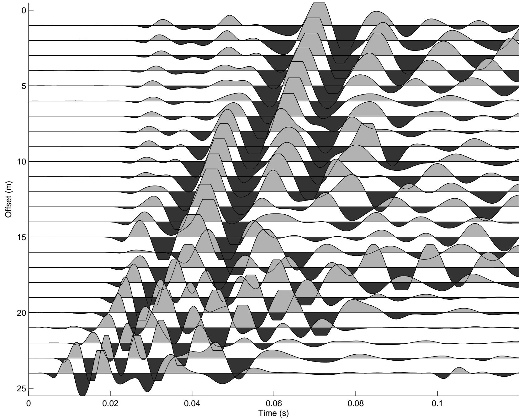
1009.dat filtered in band 50–150Hz
