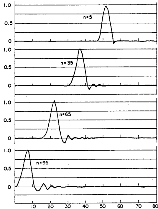
Fig. 3. Results of the calculation of E_z by means of (14a)-(14c) in the absence of the obstacle. The ordinate is in volts/meter and the abscissa is the number of horizontal increments. n is the number of time cycles.
