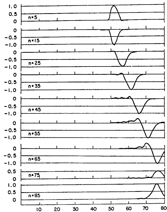
Fig. 5. E_z of the TM wave for various time cycles. j=50 .
