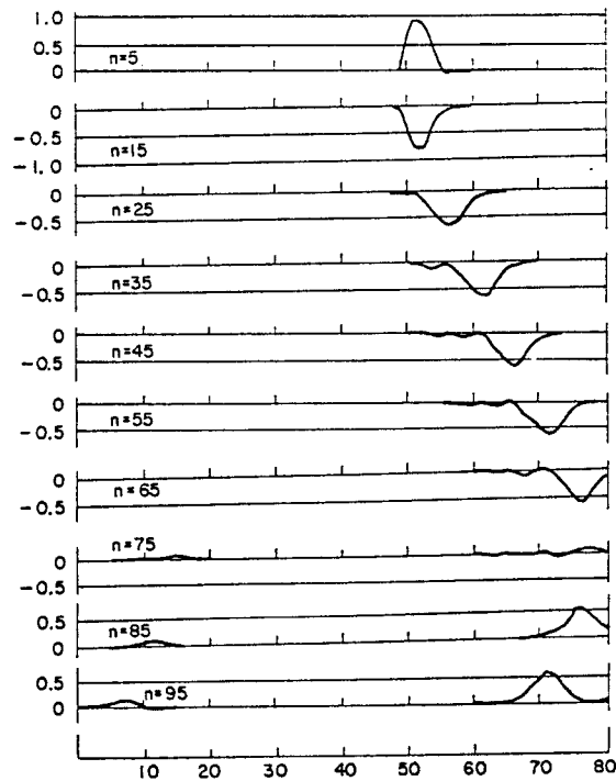
Fig. 6. E_z of the TM wave for various time cycles. j=65 .
