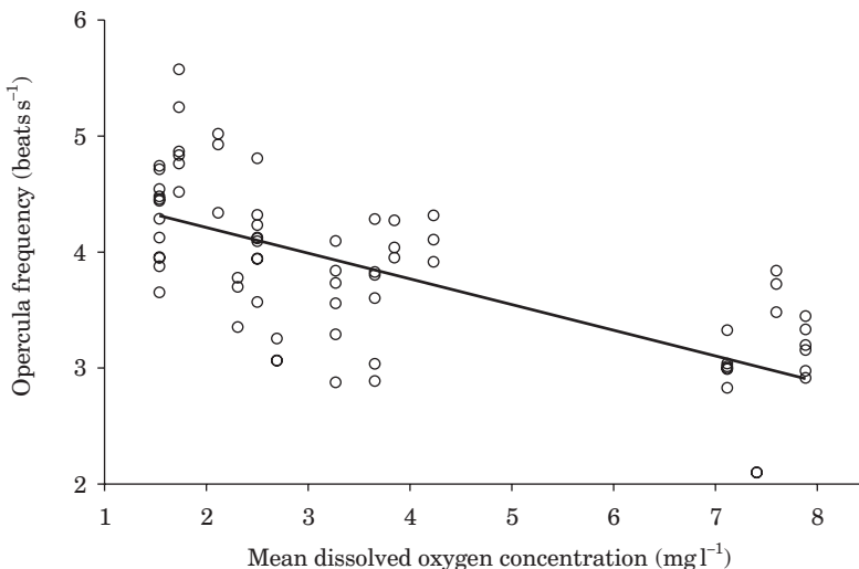
FIG. 4. Influence of mean dissolved oxygen on the mean ventilation frequency for each fathead minnow observed ( n=72 ). The line was fitted by y = -0.2215x + 4.6546 ( r^2=0.4734 , P<0.05 ).
