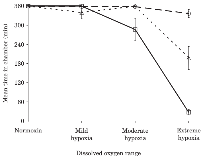
FIG. 2. Mean \pm S.E. time spent in the chamber for fathead minnow ( \circ , 2.73 \pm 0.07 g), small yellow perch ( \Delta , 2.29 \pm 0.25 g) or large yellow perch ( \square , 34.07 \pm 1.28 g) at each of the dissolved oxygen ranges tested (see text for values). Times <360 min indicate individuals were removed when they lost equilibrium.
