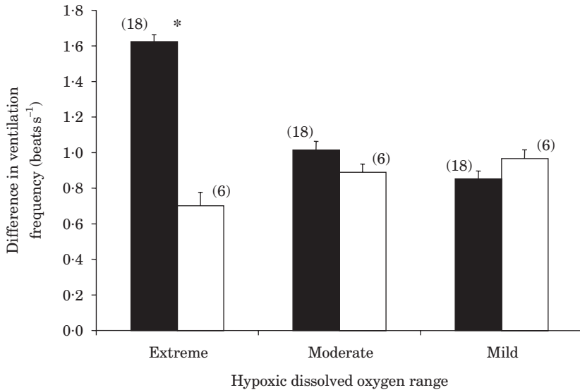
FIG. 5. Mean \pm s.e. difference from normoxic values of ventilation frequency for fathead minnow (■) and yellow perch (□) at hypoxic dissolved oxygen ranges tested (see text for values). Sample sizes used for comparison are given in parentheses. *, Significantly different between species at P < 0.05 .
