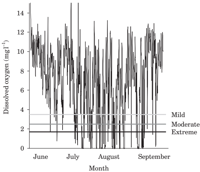
FIG. 1. Dissolved oxygen concentrations within Delta Marsh, Manitoba during the summer of 2000. Data were acquired using a YSI 6920 sonde equipped with a dissolved oxygen probe (Yellow Springs Instruments, Yellow Springs, OH, U.S.A.). Readings were taken every 10 min and averaged to provide a 1 h value. The horizontal lines represent the middle dissolved oxygen levels used for experiments.
