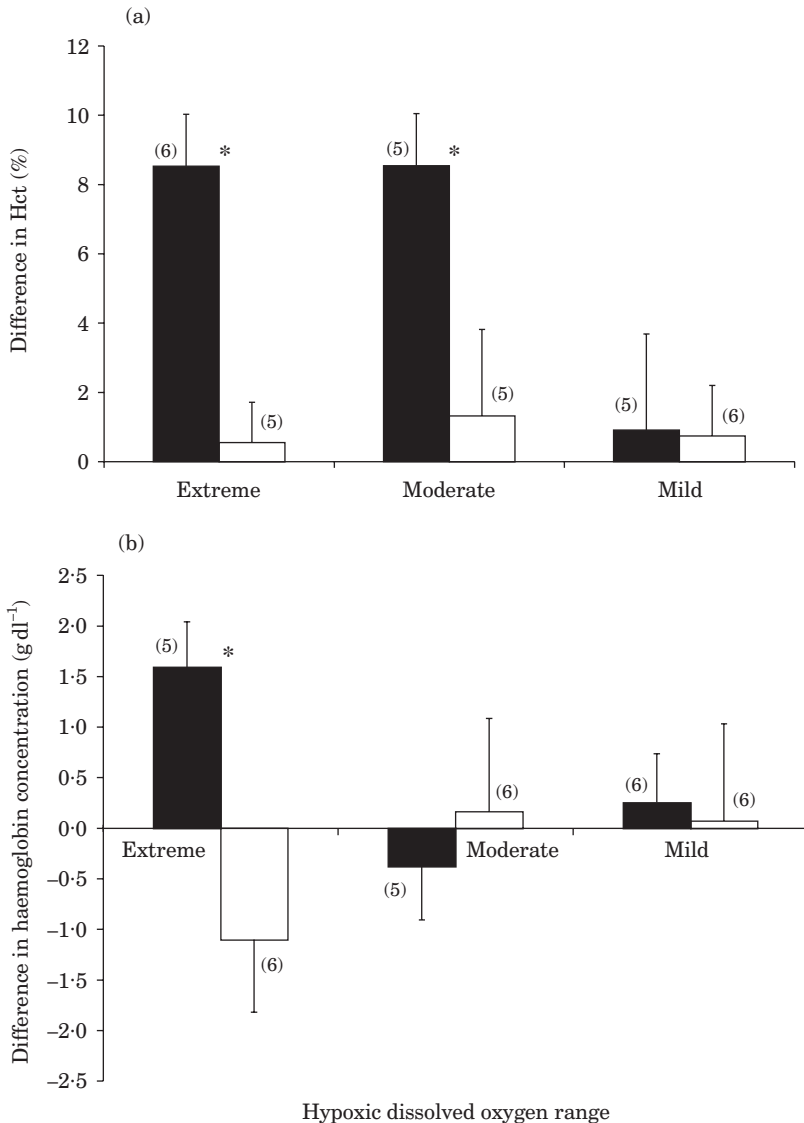
FIG. 3. Mean \pm s.e. difference from normoxic values of (a) haematocrit and (b) haemoglobin concentration for fathead minnow (■) and yellow perch (□) at hypoxic dissolved oxygen ranges tested (see text for values). Sample sizes used for comparison are indicated in parentheses. *, Significantly different between species at P < 0.05 .
