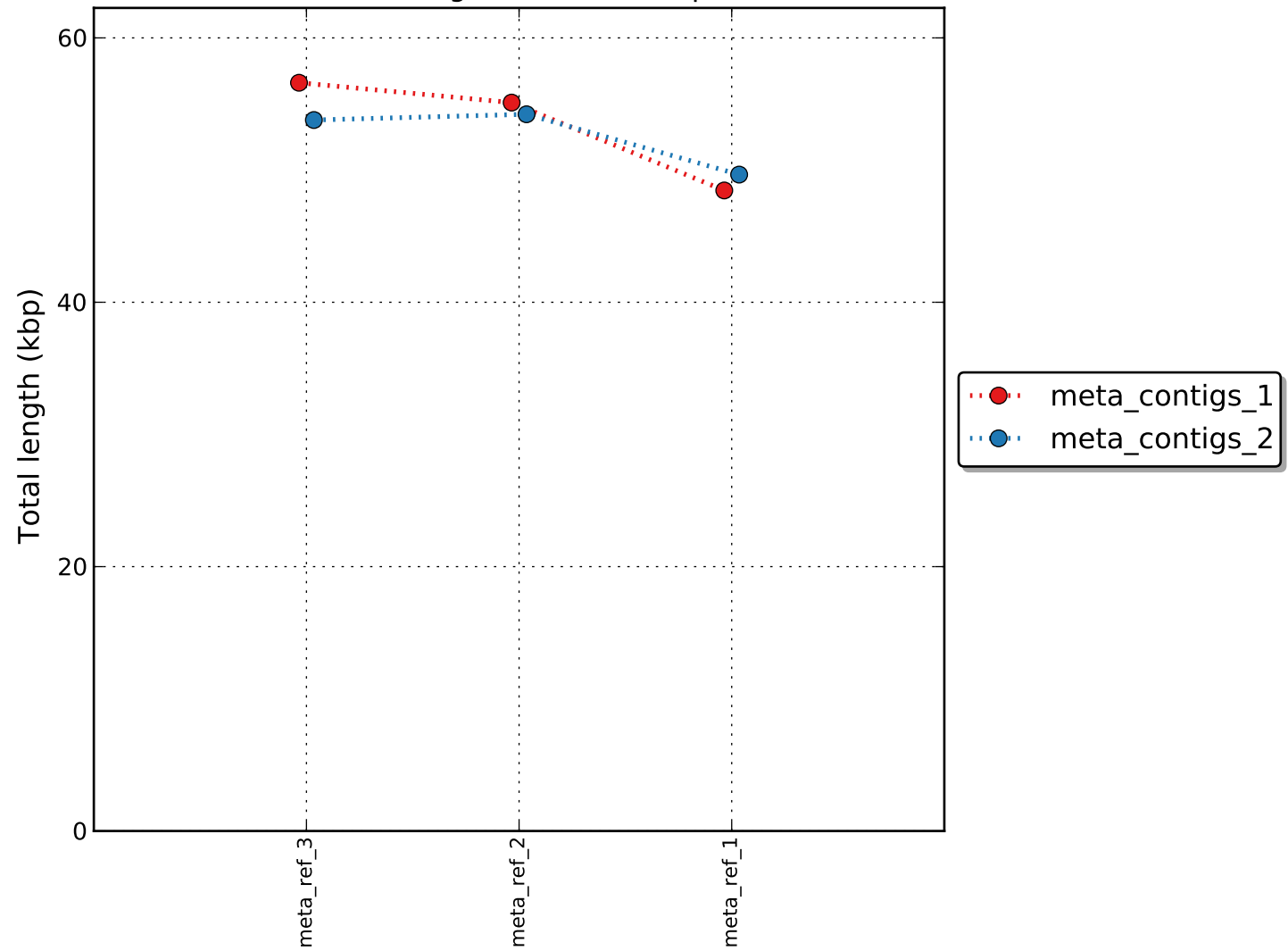
Total length ( \geq 10000 bp)
