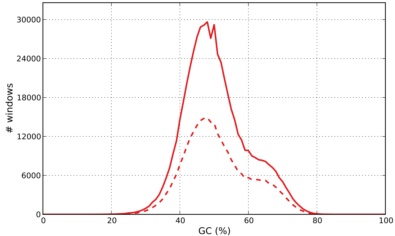
GC content
