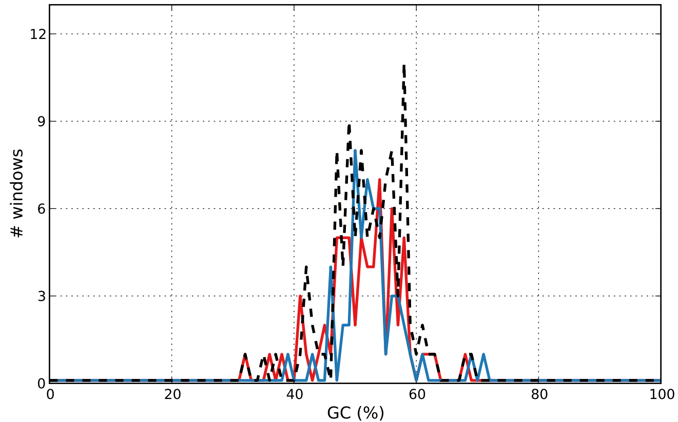
GC content
