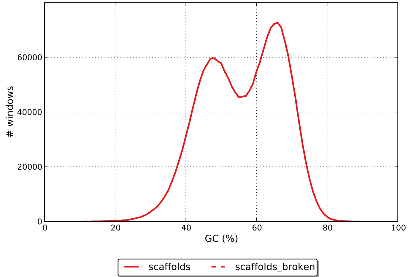
GC content
