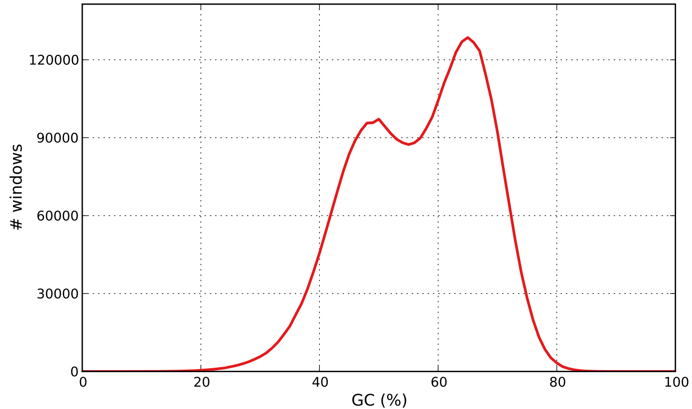
GC content
