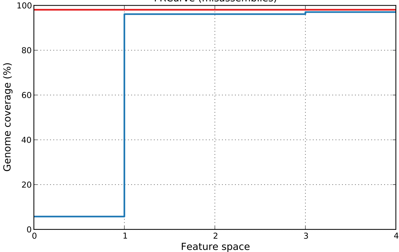
FRCurve (misassemblies)
